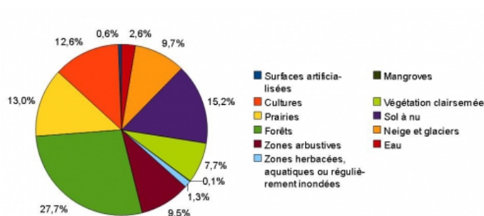
GLC-SHARE distribution of land cover types
